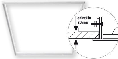
JUNA MOUNTING FRAME 600 FM WH 41 541 07
